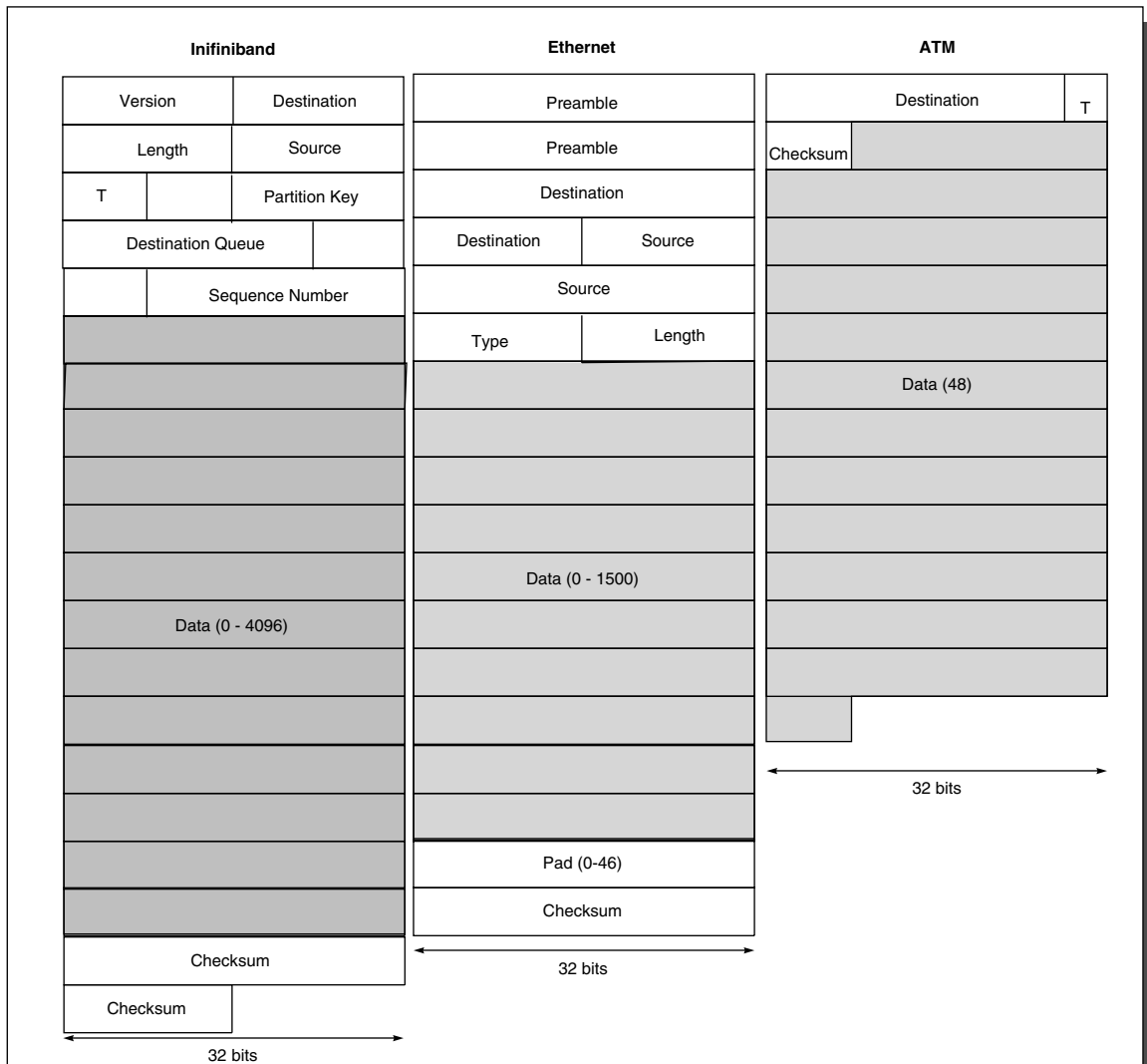
FIGURE 8.20 Packet format for Infiniband, Ethernet, and ATM. ATM calls their messages “cells” instead of packets” so the proper name is ATM cell format. The width of each drawing is 32 bits. All three formats have destination addressing fields, encoded differently for each situation. All three also have a checksum field to catch transmission errors, although the ATM checksum field is calculated only over the header; ATM relies on higher-level protocols to catch errors in the data. Both Infiniband and Ethernet have a length field, since the packets hold a variable amount of data, with the former counted in 32-bit words and the latter in bytes. Infiniband and ATM headers have a type field (T) that gives the type of packet. The remaining Ethernet fields are a preamble to allow the receiver to recover the clock from the self-clocking code used on the Ethernet, the source address, and a pad field to make sure the smallest packet is 64 bytes (including the header). Infiniband includes a version field for protocol version, a sequence number to allow in-order delivery, a field to select the destination queue, and a partition key field. Infiniband has many more small fields not shown and many other packet formats; above is a simplified view. ATM’s short packet, fixed is a good match to real-time demand of digital voice
