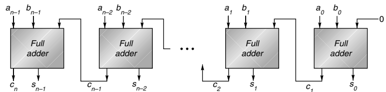
Figure H.1 Ripple-carry adder, consisting of n full adders. The carry-out of one full adder is connected to the carry-in of the adder for the next most-significant bit. The carries ripple from the least-significant bit (on the right) to the most-significant bit (on the left).
